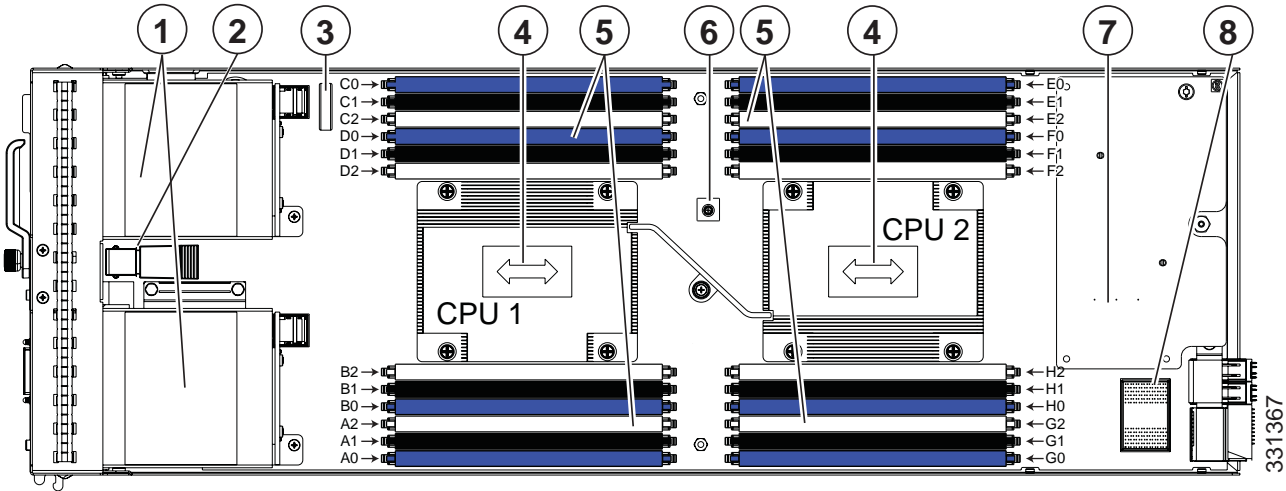
Figure 5 UCS B200 M3 System Board
